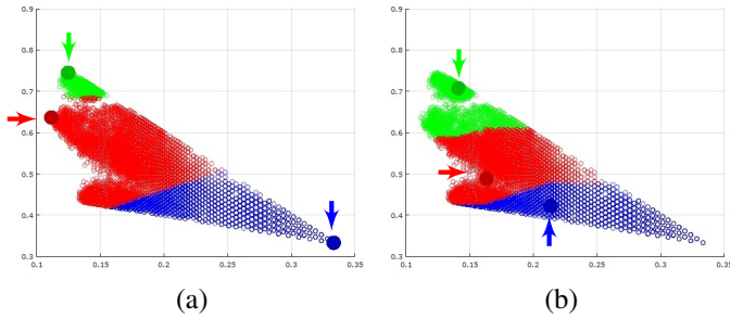
Fig. 2. Our clustering approach for the minimum ( x -axis)-maximum ( y -axis) chromaticity space. In the first iteration of our algorithm (a), we select three cluster seeds (big circles pointed by arrows) located at the highest minimum (blue circle), highest maximum (green circle), and lowest minimum chromaticity values (red circle). Then, we run two iterations of k -means to associate each pixel to the nearest cluster seed in the Euclidean space, update the position of the cluster seeds according to the centroid of their associated pixels, and associate each pixel on the basis of the updated cluster seeds (b).
